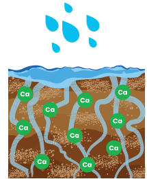
Flocculated Soil
